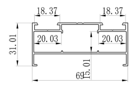
Perimeter J6901
