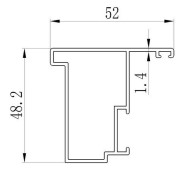
Adapter 45G07
