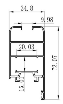
Panel J6903
